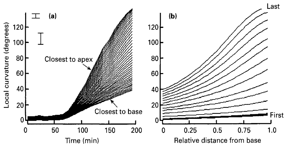
Fig. 13. The distribution of local curvature over the length of the stem for Coprinus cinereus stems treated with A231817 (1 \mu M, 2 h). (a) Time-telescoped projection (each curve represents the changing curvature of a different stem subsection); (b) space-telescoped projection (curves represent 10 min time intervals). The distance from the base is given in arbitrary units of stem length. The error bar at the top left of (a) represents maximum SD for both projections. Note that stem straightening was minimal.
