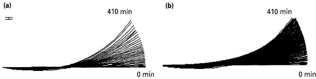
Fig. 12. Comparison of (a) averaged bending of Coprinus cinereus stems treated with cytochalasin D (10 \mu M, 2 h) with (b) the images generated by the model shown as Eqn 7 with parameters given in Table 3. In (b), computer-generated images (thick lines) are plotted over, and because of the accuracy of the model largely obscure, the experimentally observed images (regular lines). Times of subsequent images differ by 10 min. The error bar at the top left of (a) defines the maximum SD of the mean for experimentally observed shapes. The goodness of fit was tested by the lack-of-fit test (see Table 1).
