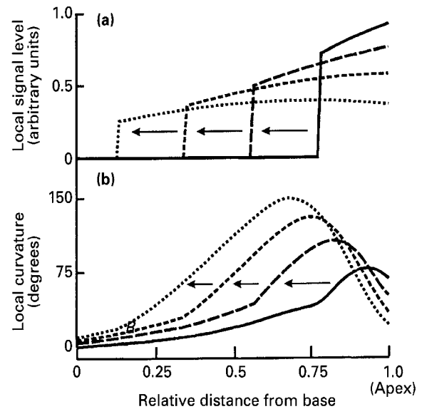
Fig. 2. Computer-generated distribution of the local level of the hypothetical gravitropic signal perceived in the apex (a) and the local curvature (b) during simulation of the gravitropic reaction of Coprinus cinereus stems. During the bending process the apex angle, and hence the signal level in the apex, decreases. The simulation was performed with parameter values from Table 2. The curvature distribution (b) can also be compared with directly measured data (Fig. 5b).
