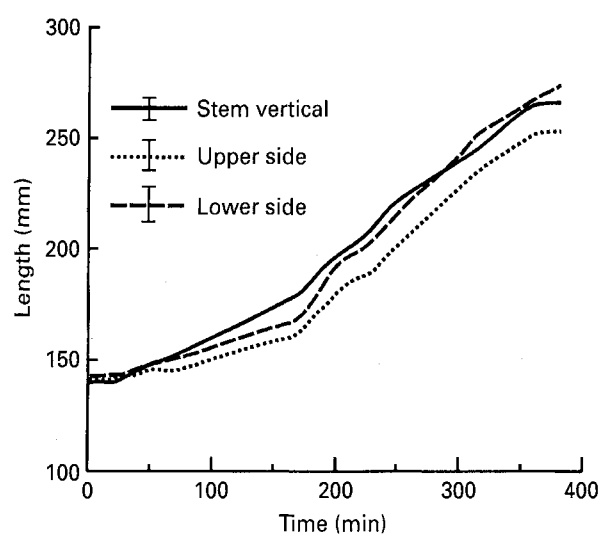
Fig. 4. The growth of the upper and lower sides of Coprinus cinereus stems during the gravitropic reaction. Growth was measured for the whole length of each side. The error bars in the upper part of the figure represent the maximum SD of the mean for each curve.
